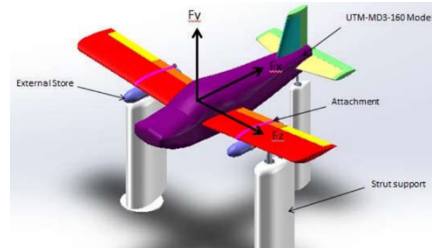
Figure 1: Experimental rig for light aeroplane in 3-axis gauge sensor.
