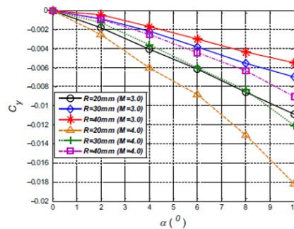
Figure 2: Value of C_y vs angle of attack.
